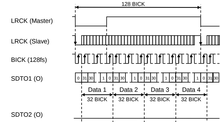
Figure 45. Mode 27/31 Timing (TDM128 mode, I²S Compatible)
