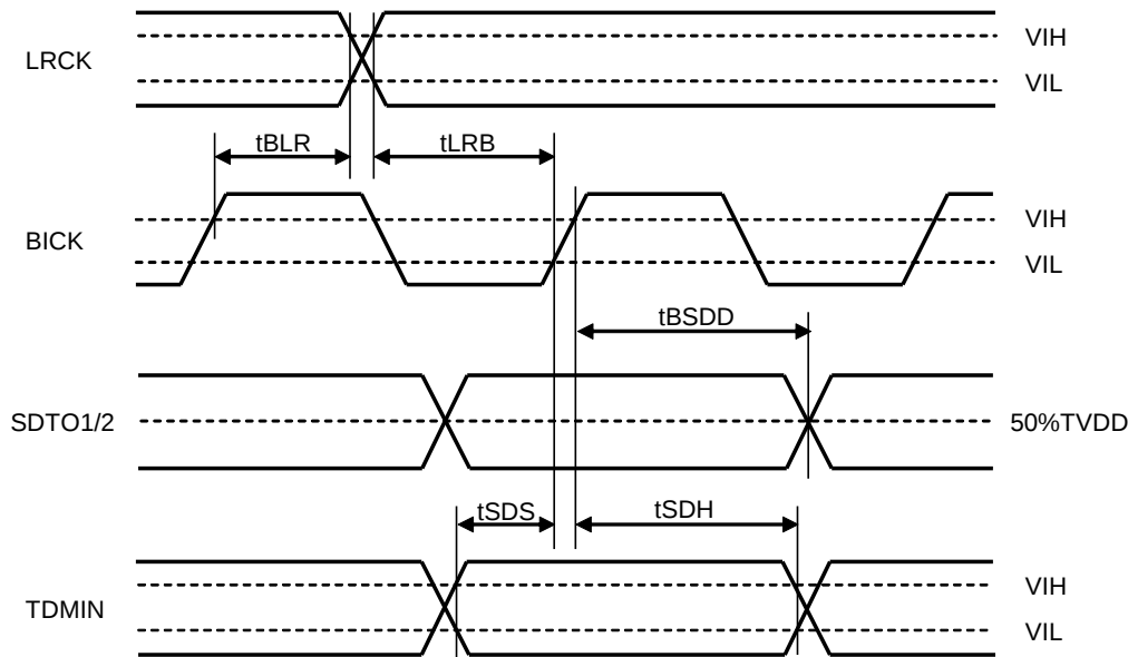
Figure 21. Audio Interface Timing (TDM & Slave mode)
