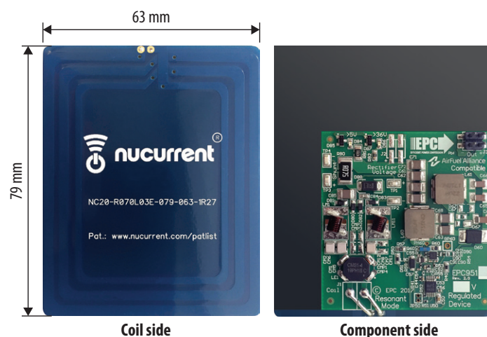
Figure 1: Photo of the EPC9513 receiver board.
