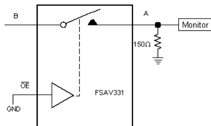
FIGURE 5. Bandwidth Test
