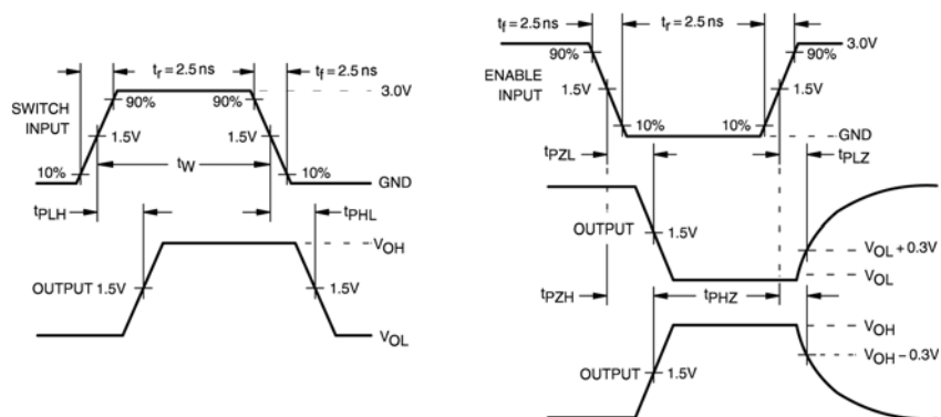
FIGURE 2. AC Waveforms
