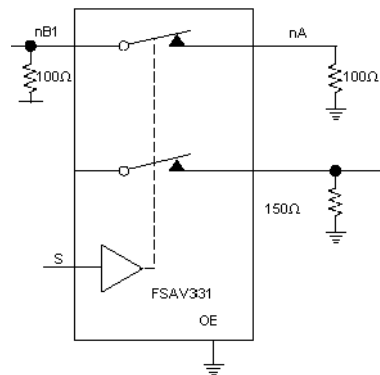
FIGURE 4. Crosstalk Test
