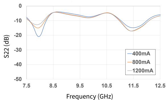
Figure 42. Output RL vs Frequency as a Function of I_{DQ}
