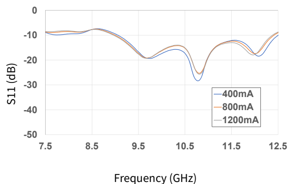
Figure 40. Input RL vs Frequency as a Function of I_{DQ}
