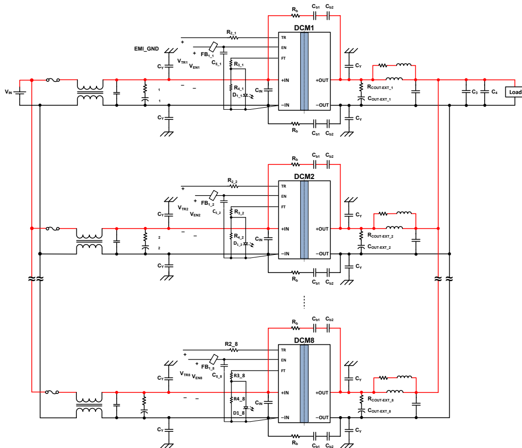
Figure 30 — DCM paralleling configuration circuit 2
