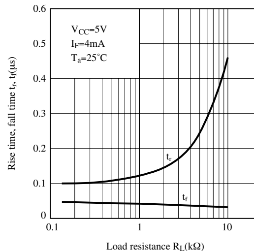
Fig.14 Rise Time, Fall Time vs. Load Resistance
