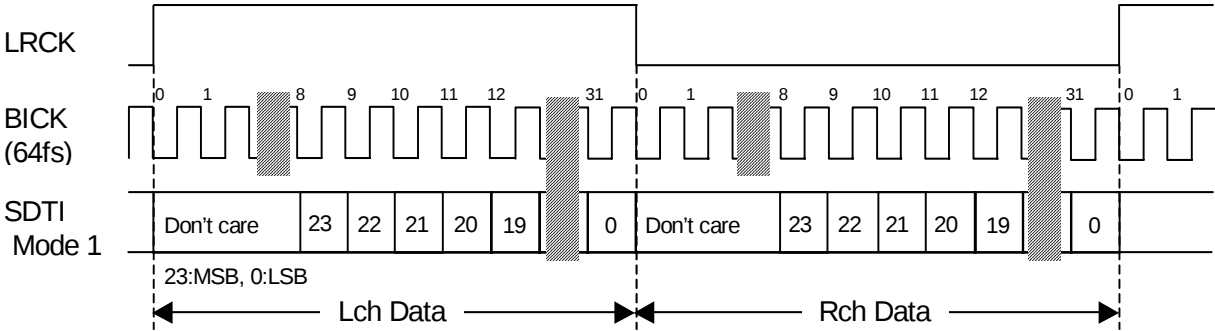
Figure 5. Mode 1 Timing
