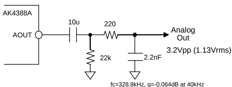
Figure 12. External 1 st order LPF Circuit Example (simple)
