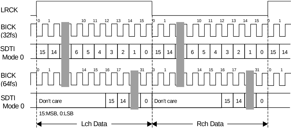
Figure 4. Mode 0 Timing
