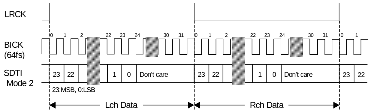
Figure 6. Mode 2 Timing
