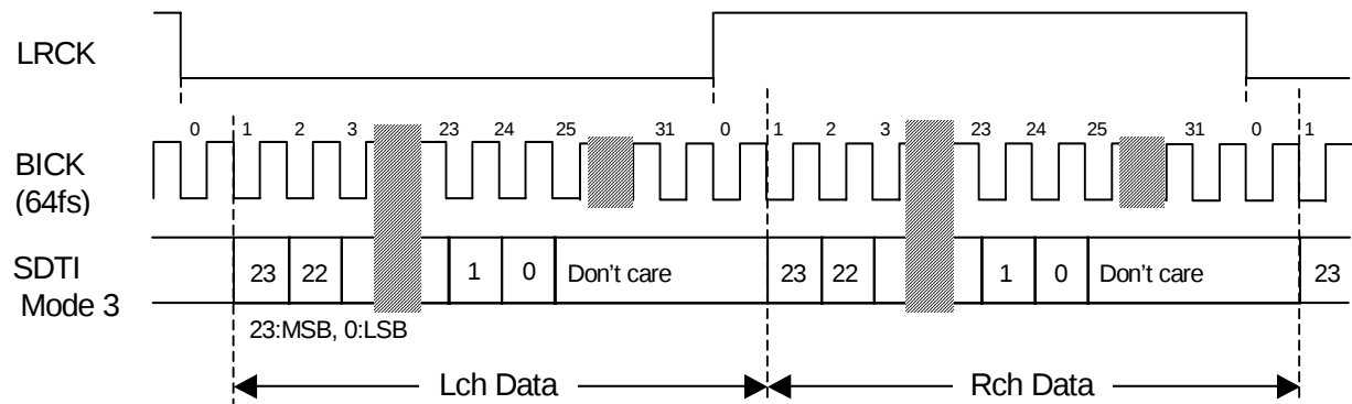
Figure 7. Mode 3 Timing
