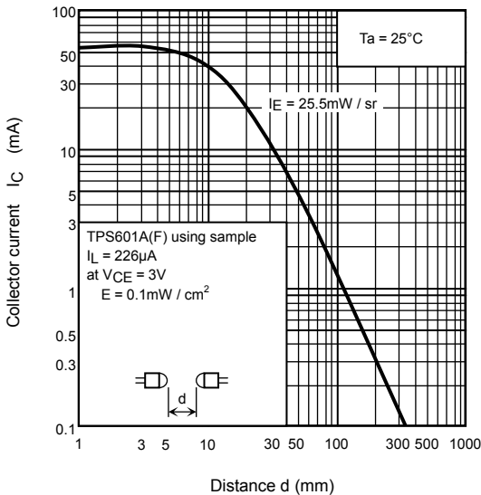
Coupling Characteristic With TPS601(F)
