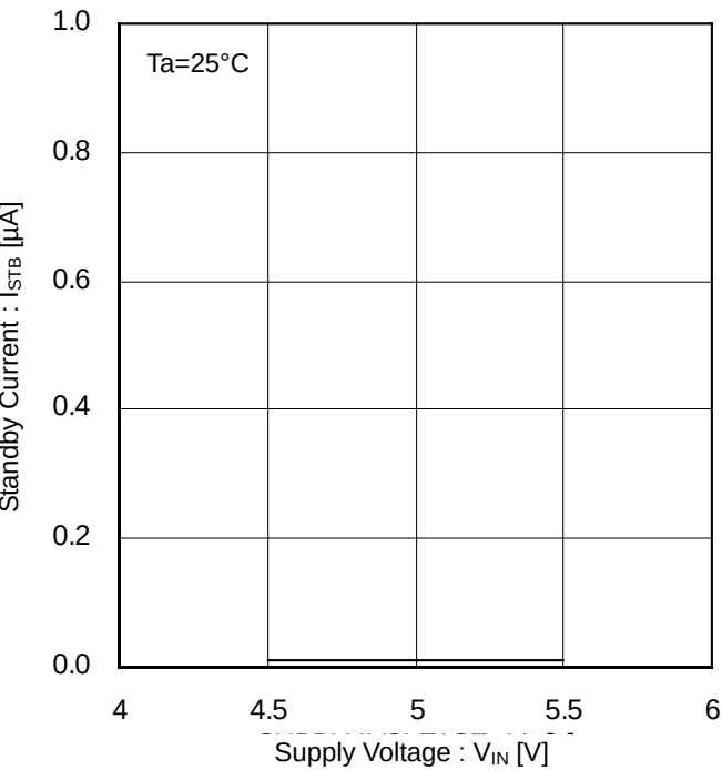
Figure 8. Standby Current vs Supply Voltage EN Disable
