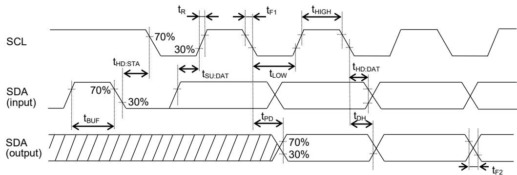
○Input read at the rise edge of SCL ○Data output in sync with the fall of SCL Figure 5-(a). Input/Output Timing
