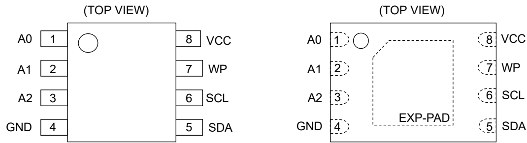
Figure 3-(a). Pin Configuration (SOP8 *1 , SOP-J8, TSSOP-B8, MSOP8) *1 Last Time Buy. Figure 3-(b). Pin Configuration (VSON08AX2030)
