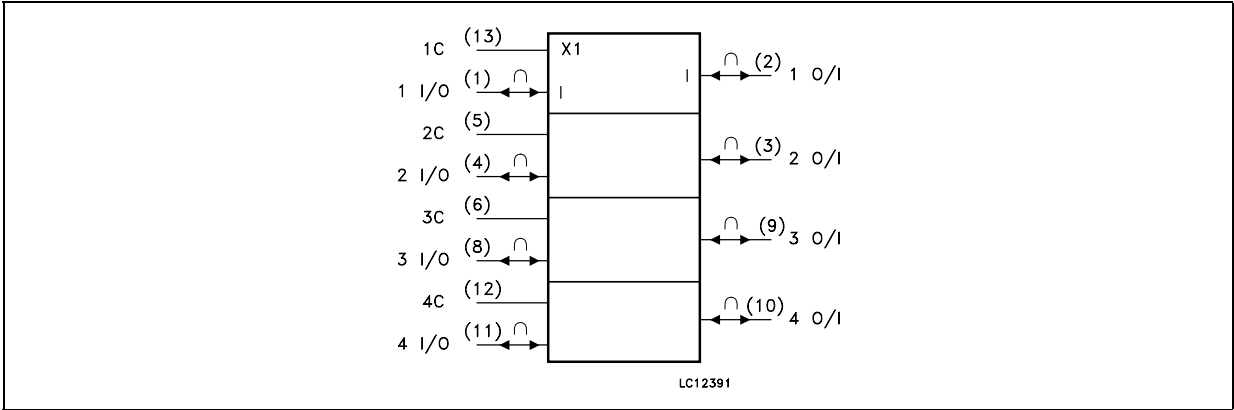
Figure 2: Logic Diagram
