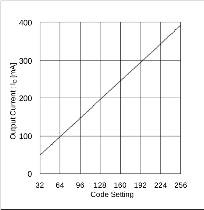
Figure 10. Output Current vs Code Setting (Current Driver Block, R_{RNF}=1.0\ \Omega , R_L=5.0\ \Omega )
