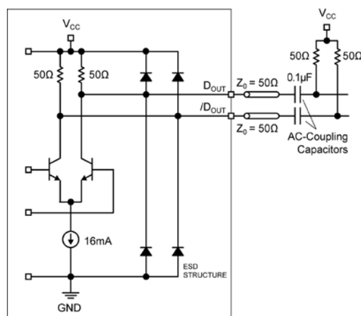
Figure 3. Output Structure
