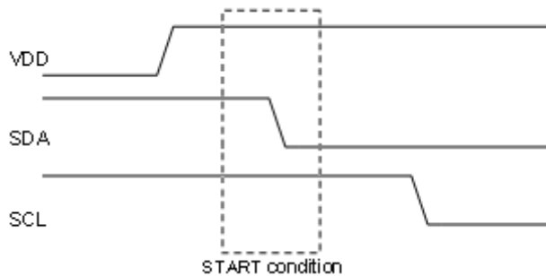
Figure 25. Start Condition
