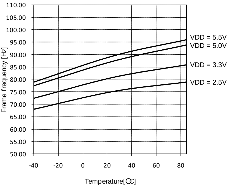
Typical temperature characteristics
