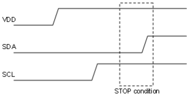
Figure 24. Stop Condition
