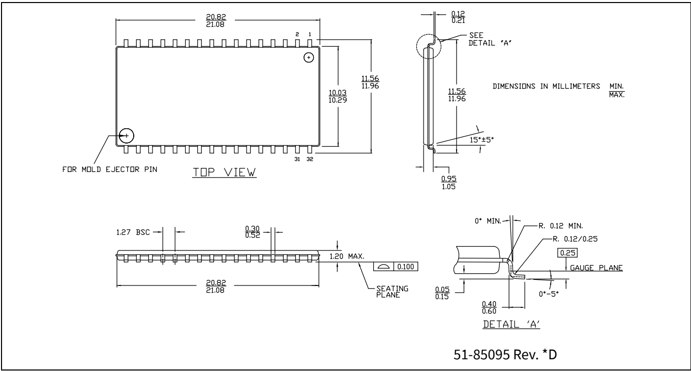
Figure 11 32-pin TSOP II (20.95 × 11.76 × 1.0 mm) ZS32 package outline (PG-TSOP-32), 51-85095
