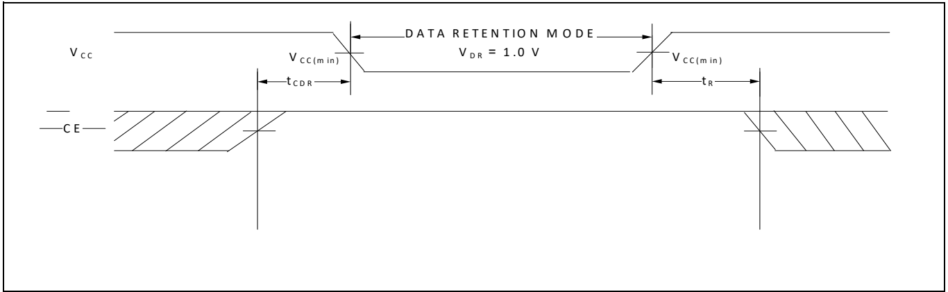
Figure 4 Data retention waveform
