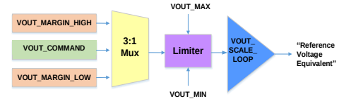
Figure 7: Reference Voltage Setting
