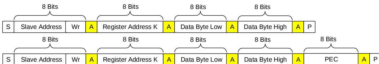
Figure 13: Write Word without PEC and Write Word with PEC
