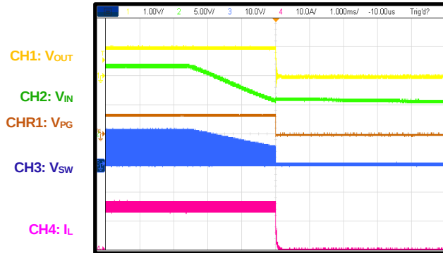
Shutdown through the Input Voltage I_{OUT} = 15A
