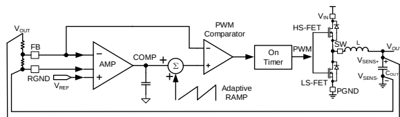
Figure 3: COT Control
