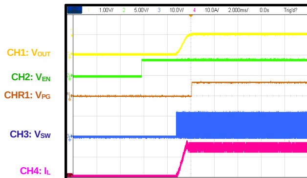
Start-Up through EN I_{OUT} = 15A
