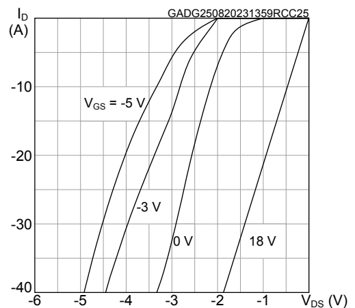
Figure 8. Typical reverse conduction characteristics ( T_J = 25^\circ\text{C} )
