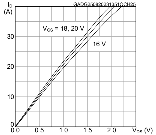
Figure 4. Typical output characteristics ( T_J = 25^\circ\text{C} )
