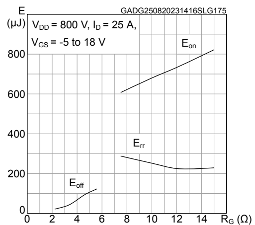
Figure 14. Typical switching energy vs gate resistance ( T_J = 175^\circ\text{C} )
