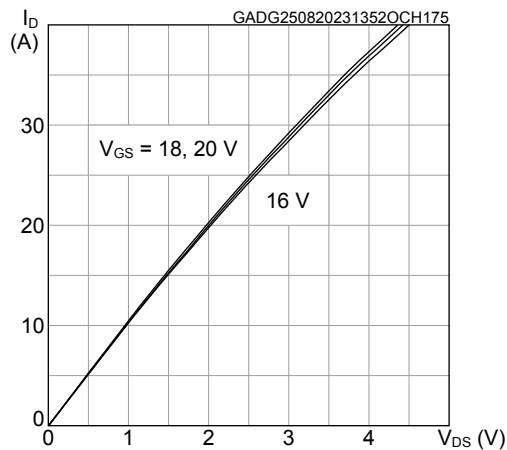
Figure 5. Typical output characteristics ( T_J = 175^\circ\text{C} )
