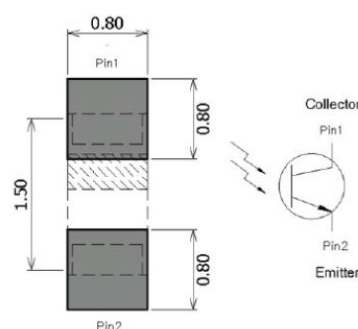
Figure 1. IN-S63DTPT Solder Pattern
