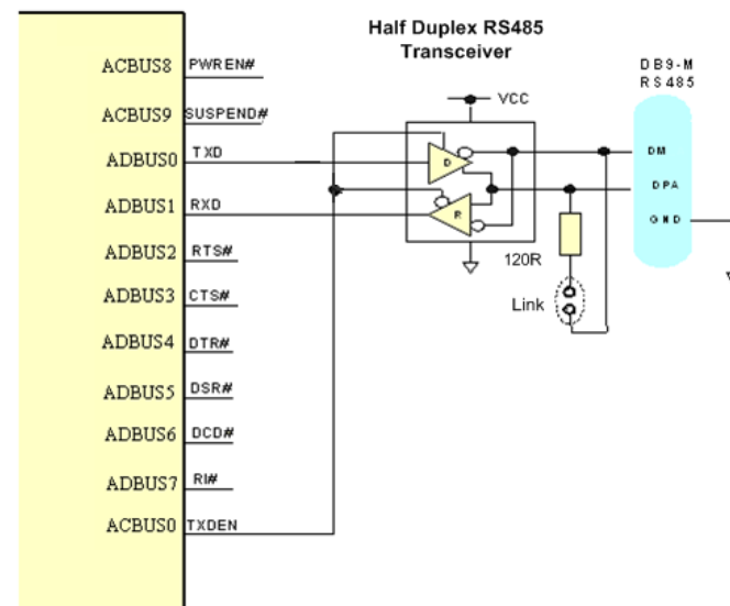
Figure 6 - RS485 Configuration
