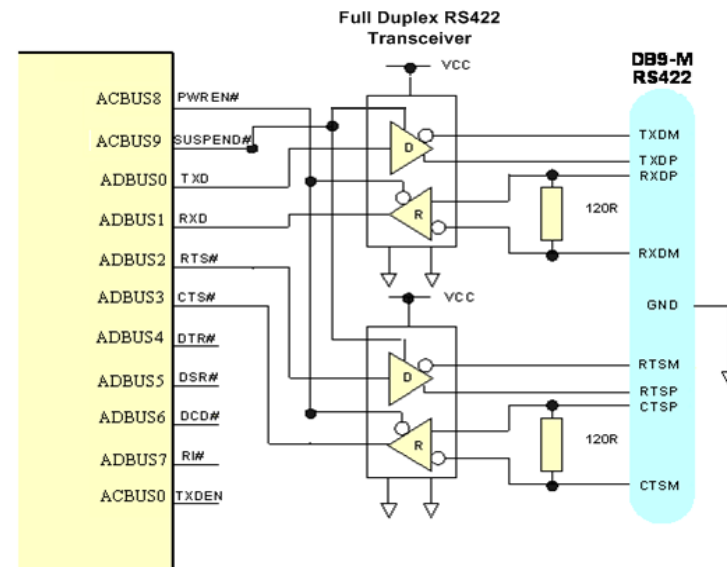
Figure 5 - RS422 Configuration
