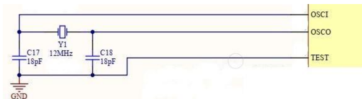
Figure 33 - Recommended FT233HP/FT232HP Crystal Oscillator Configuration
