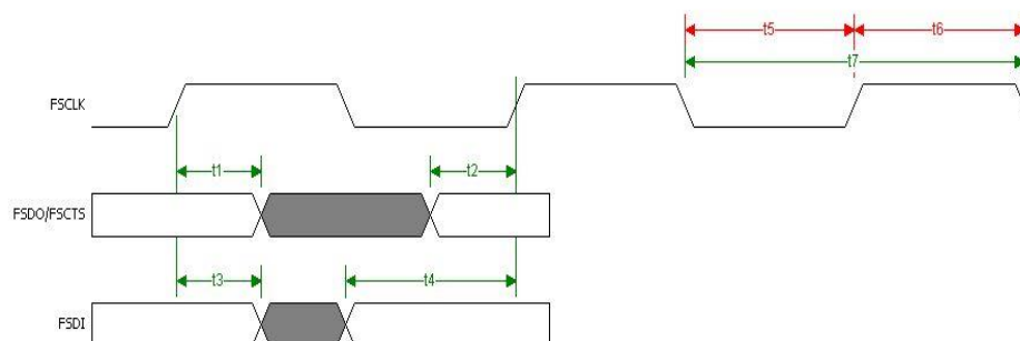
Figure 20 - Fast Serial Interface Signal Waveforms
