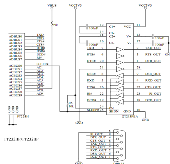
Figure 4 - RS232 Configuration
