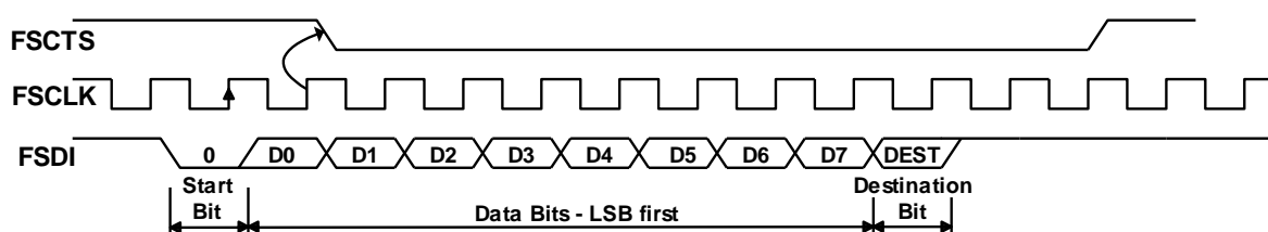
Figure 22 - Fast Serial Interface Input Data
