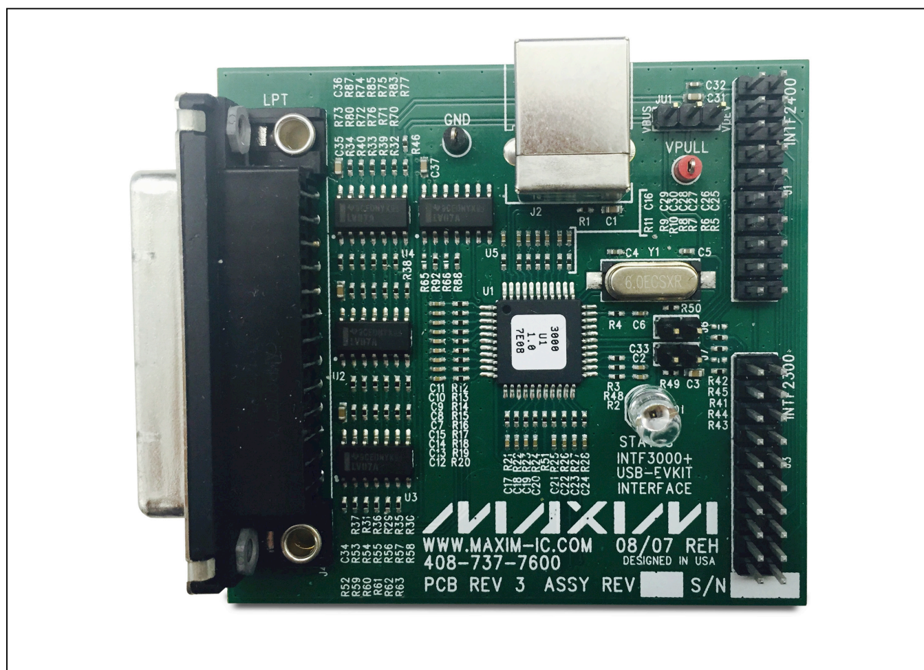
Figure 1. INTF3000 Board
