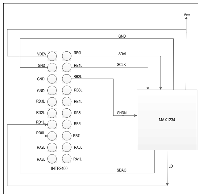
Figure 10. 4-Wire Serial Communication Example Schematic
