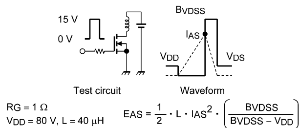
Fig. 8.17 Test Circuit/Waveform
