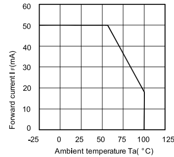
Fig. 7 Forward Current vs. Ambient Temperature
