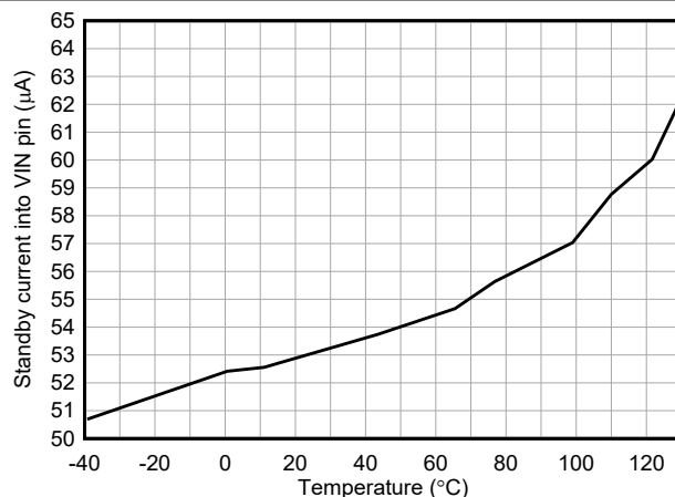
Figure 6-18. Standby Current into VIN versus Temperature V_{EN/UVLO} = 0.8\text{ V} , V_{(VIN)} = 12\text{ V}
