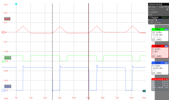
Figure 9-4. Inductor current buck-boost operation (MODE = V_{(VCC)} , V_o = 12\text{ V} , I_o = 0\text{ A} , V_{(VIN)} = 12\text{ V} )
