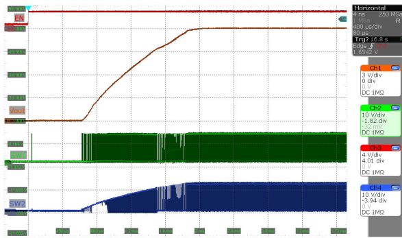
Figure 9-2. Start-up waveform standby to active operation (MODE = V_{(VCC)} , V_o = 12\text{ V} , I_o = 0\text{ A} , V_{(VIN)} = 12\text{ V} )
