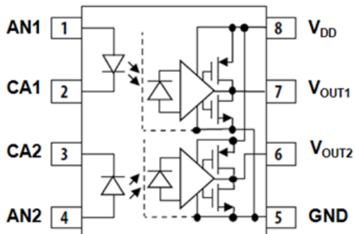
Figure 2: ACPL-K74T/ACPL-K75T
