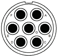
24-10 Service A 7 Contacts, Size #8 (100)
