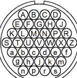
28-21 Service A 37 Contacts, Size #16 (15)
