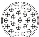
36-A22 Service D 22 Contacts, Size #12 (25)
