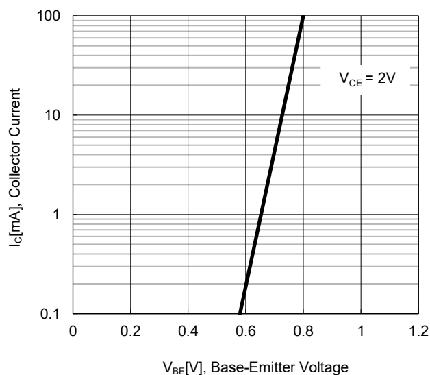
Fig.4 Base-Emitter On Voltage
