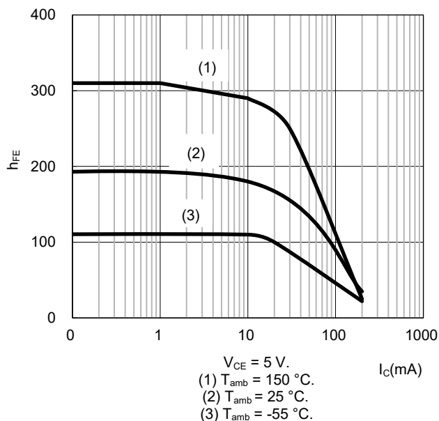
Fig. 2 DC Current Gain
