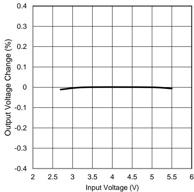
Figure 11. Line Regulation
