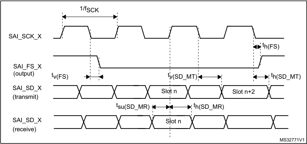
Figure 58. SAI master timing waveforms
