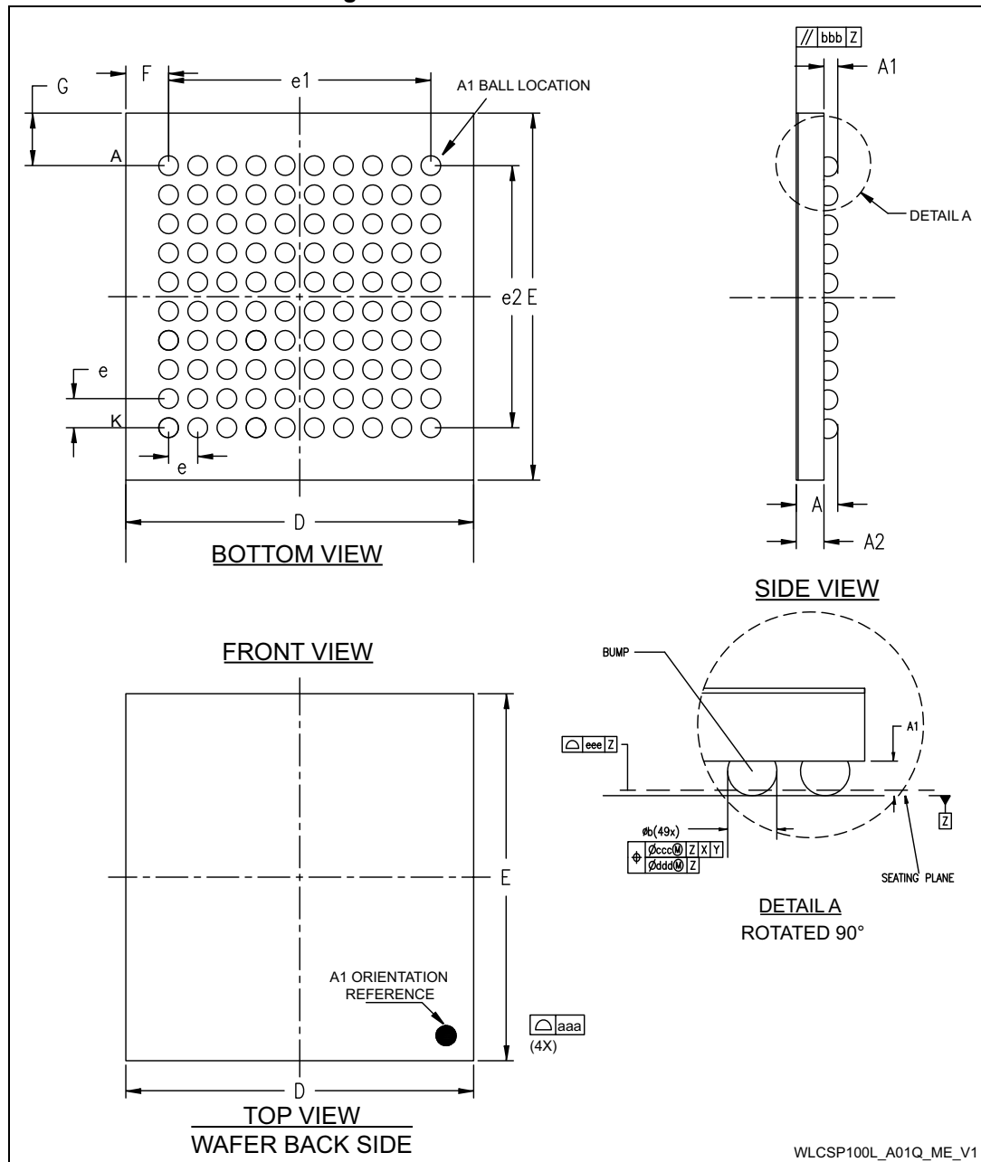
Figure 98. WLCSP100 outline
