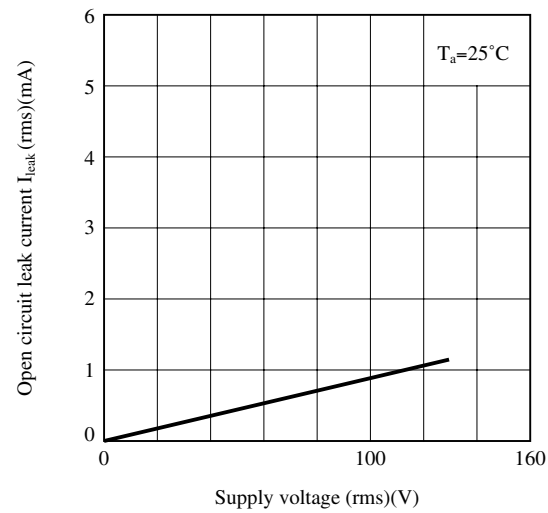
Fig.8-a Open Circuit Leak Current vs. Supply Voltage (S102S11)
