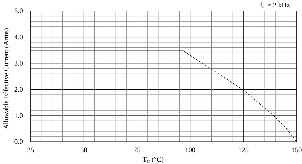
Figure 15-58. Allowable Effective Current ( f_C = 2 \text{ kHz} ): SIM6895M
