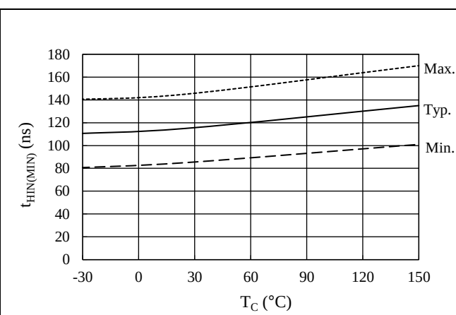
Figure 15-18. Minimum Transmittable Pulse Width for High-side Switching, t_{HIN(MIN)} vs. T_C
