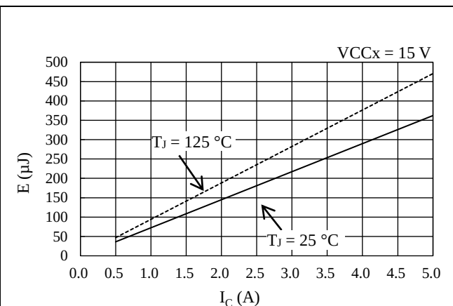
Figure 15-45. Low-side Switching Loss
