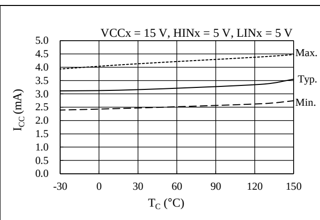
Figure 15-2. Logic Supply Current, I_{CC} vs. T_C ( I_{N_x} = 5 V)
