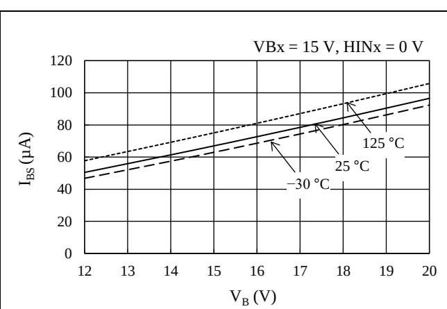
Figure 15-6. V_{Bx} Pin Voltage, V_B vs. Logic Supply Current, I_{BS} ( HIN_x = 0 V)
