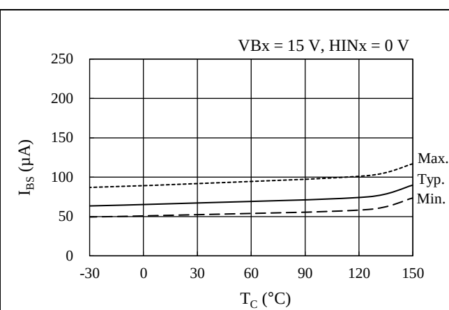
Figure 15-4. Logic Supply Current (1-phase) I_{BS} vs. T_C ( HIN_x = 0 V)
