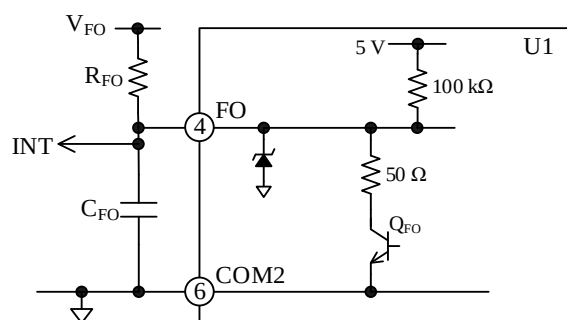
Figure 12-9. Internal Circuit Diagram of FO Pin and Its Peripheral Circuit
