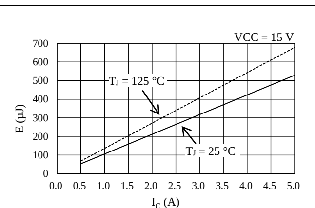
Figure 15-47. Low-side Switching Loss
