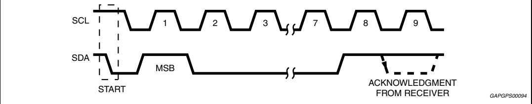
Figure 27. Timing acknowledge clock pulse
