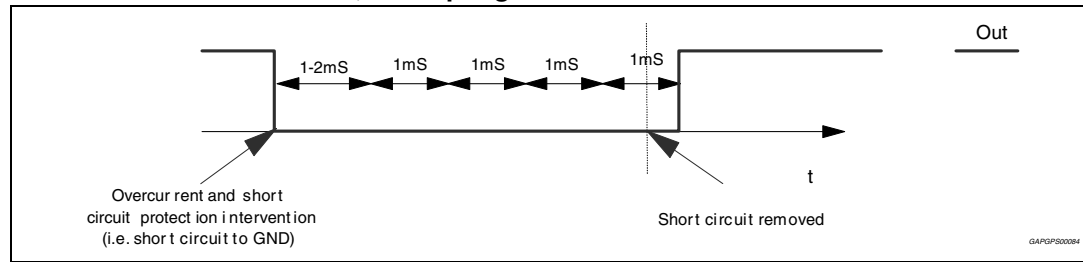
Figure 23. Restart timing with diagnostic enable (permanent)
