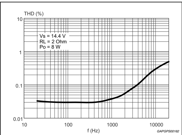
Figure 9. Distortion vs. frequency (2 Ω)
