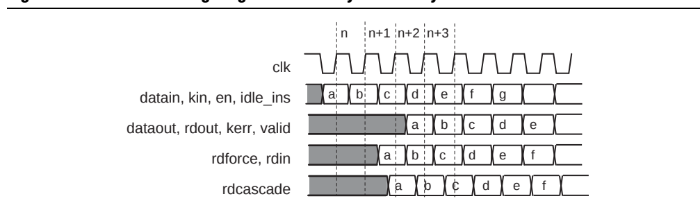
Figure 3–5. Encoder Timing Diagram—Three Cycle Latency
