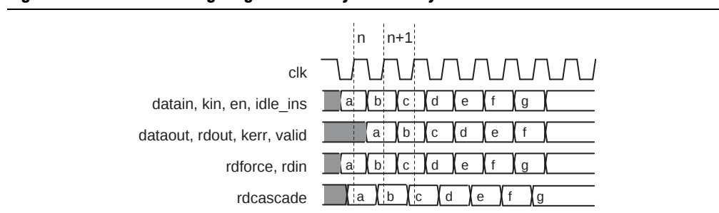
Figure 3–6. Encoder Timing Diagram—One Cycle Latency
