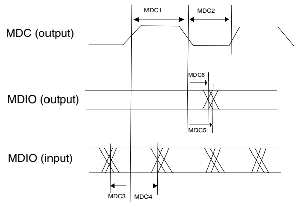
Figure 28. MII/RMII serial management channel timing
