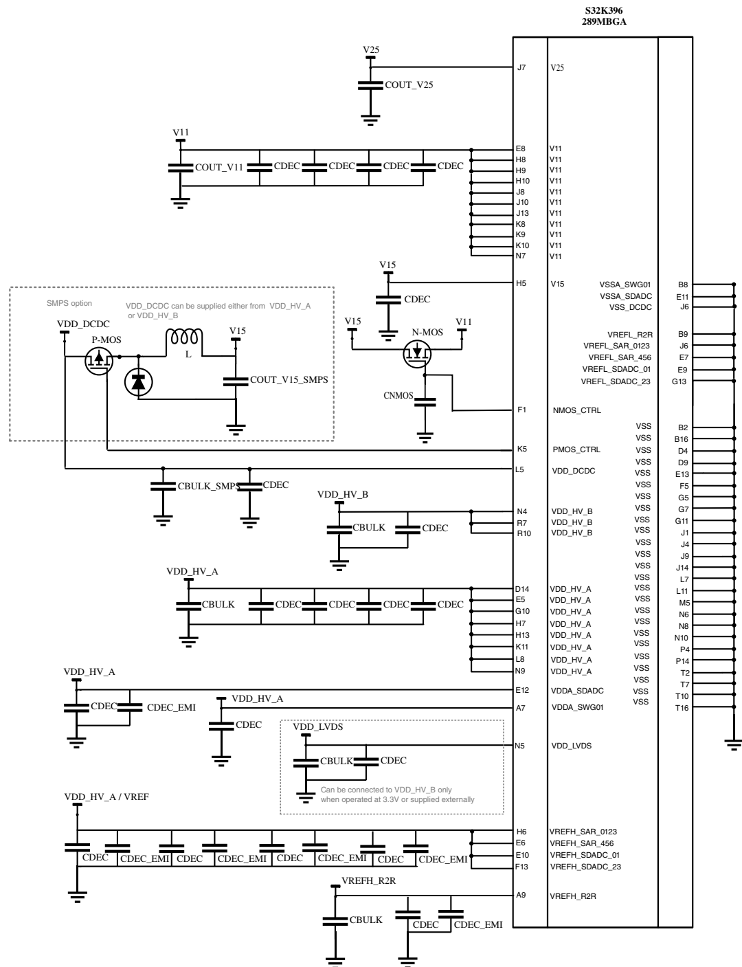
Figure 8. 289BGA decoupling capacitor pinout diagram (SMPS)
