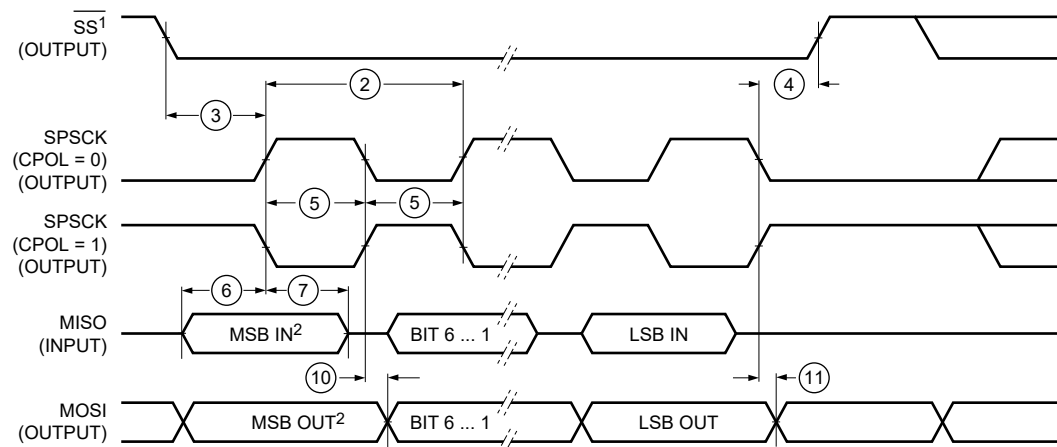
Figure 26. LPSPI Master Mode Timing (CPHA=0)
