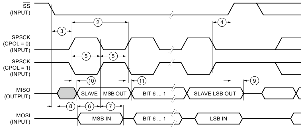
Figure 24. LPSPI Slave Mode Timing (CPHA=1)
