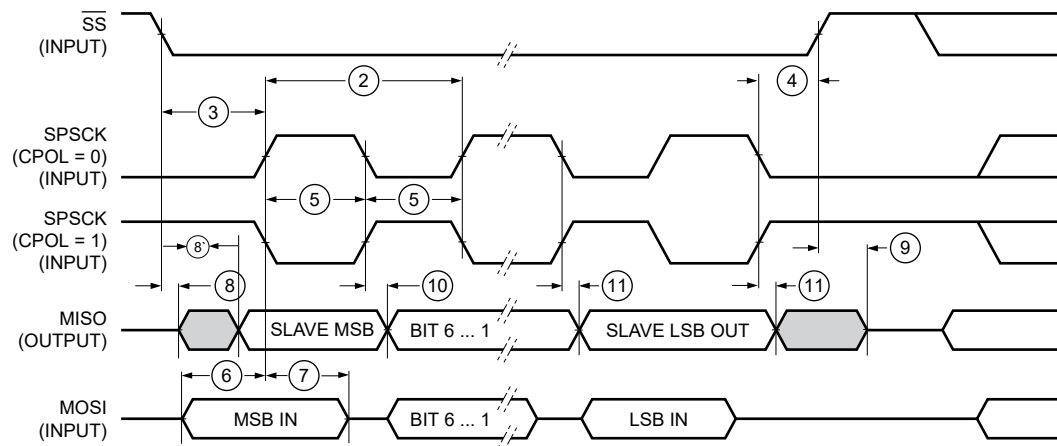
Figure 25. LPSPI Slave Mode Timing (CPHA=0)
