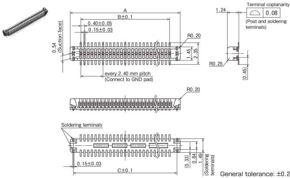
Dimension table
