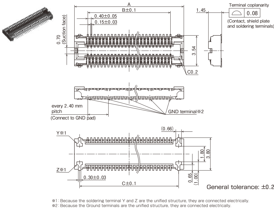
Dimension table
