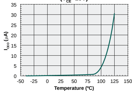
LIA135 - Dark Current vs. Temperature Measured At Pins 3&4 ( V_{CE}=10V )
