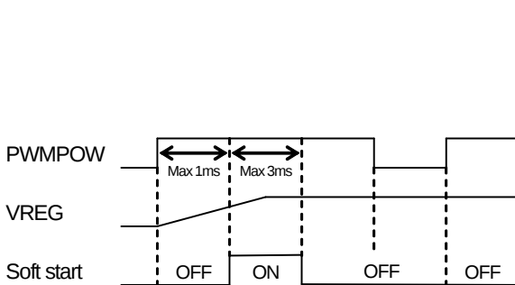
Fig.20 Soft start
