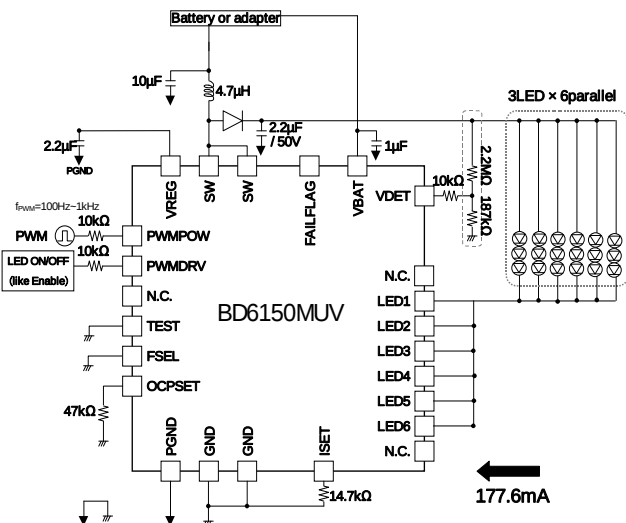
Fig.55 3series × 6parallel, LED current 177.6mA setting, Switching frequency 1250kHz setting example Power control PWM application
