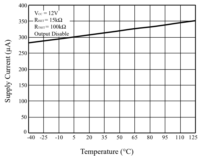
Figure 12 Supply Current vs. Temperature
