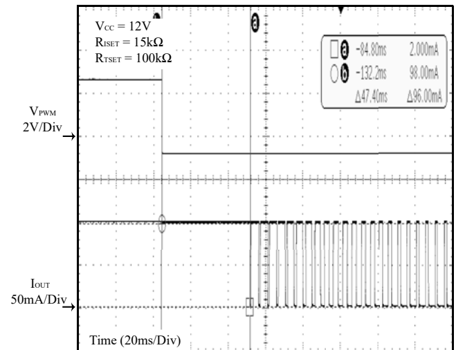
Figure 40 Internal-PWM-Dimming Off
