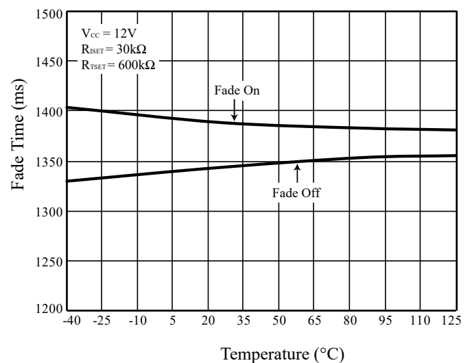
Figure 20 Fade Time vs. Temperature
