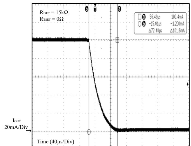
Figure 42 Instant Off
