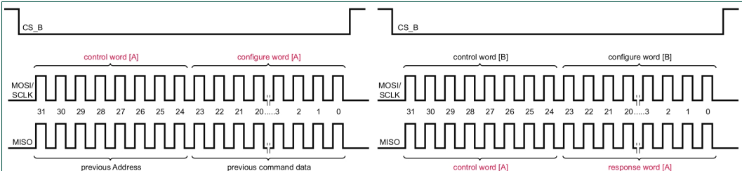
Figure 12. Full duplex SPI transaction example
