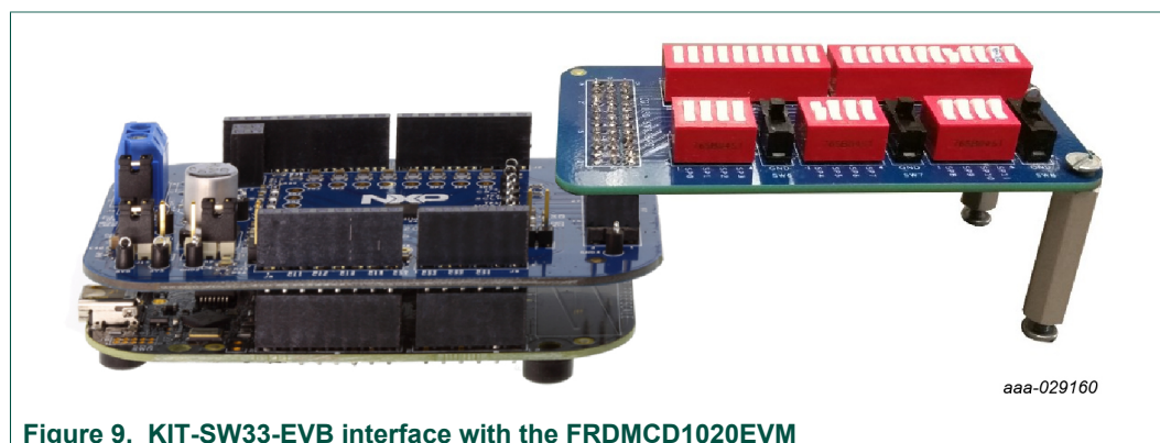
Figure 9. KIT-SW33-EVB interface with the FRDMCD1020EVM
