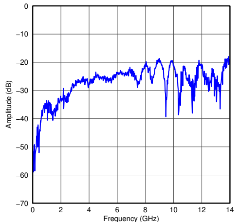
Figure 6-2. Differential to Common Mode Conversion
