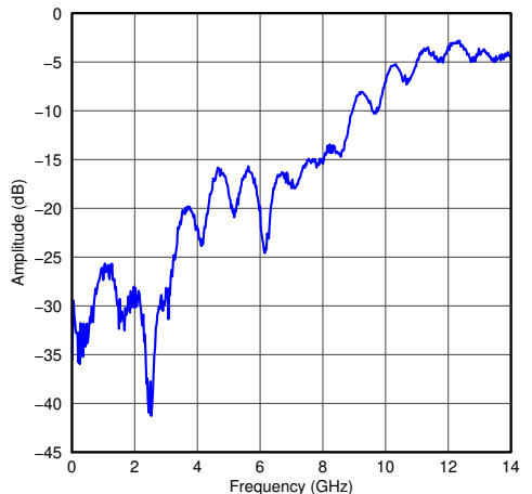
Figure 6-1. Differential Input Return Loss
