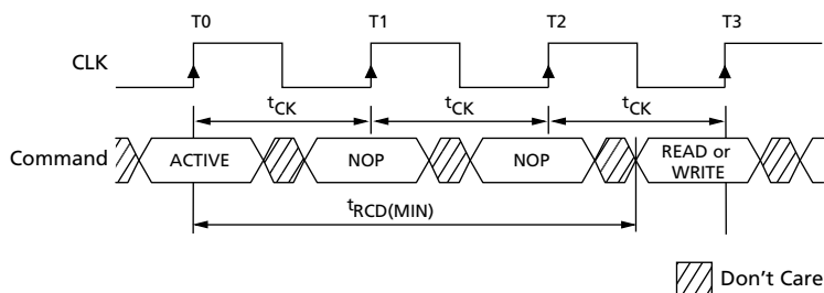
Figure 16: Example: Meeting t_{\text{RCD}}(\text{MIN}) When 2 < t_{\text{RCD}}(\text{MIN})/t_{\text{CK}} \leq 3
