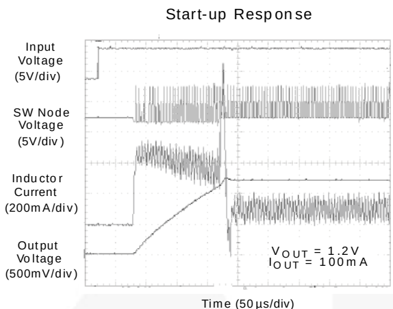
Figure 7. Startup Response
