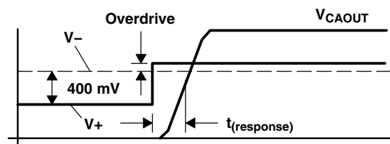
Figure 9. Overdrive Definition
