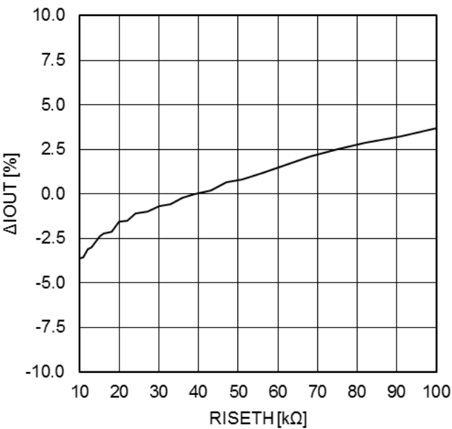
Figure 12. ΔIOUT vs RISETH (STOP=High)
