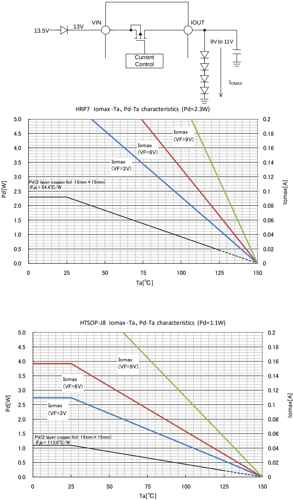
Figure 25. Heat reduction curve
