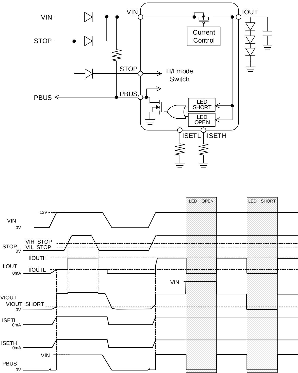
Figure 13. Timing Chart
