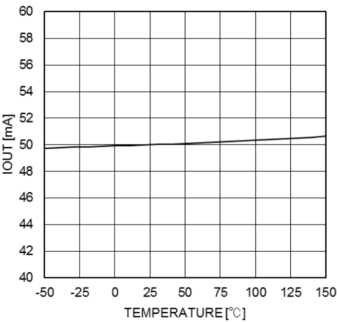
Figure 10. IOUT vs Ta (STOP=High)
