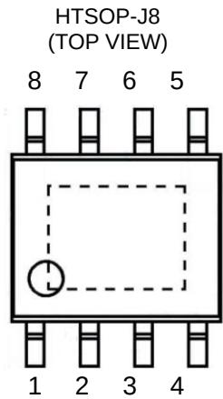
Figure 3. HTSOP-J8 Package Pin Configuration
