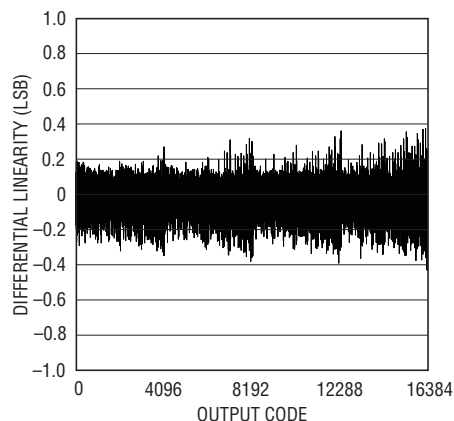
Differential Linearity for CH0 with Internal 2.5V Reference
