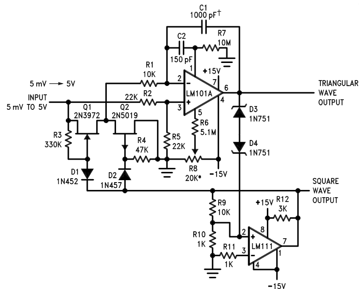
Figure 44. 100 kHz Free Running Multivibrator
