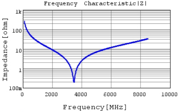
GCQ1555C1H6R1CB01 |Z| DC0V, 25degC
