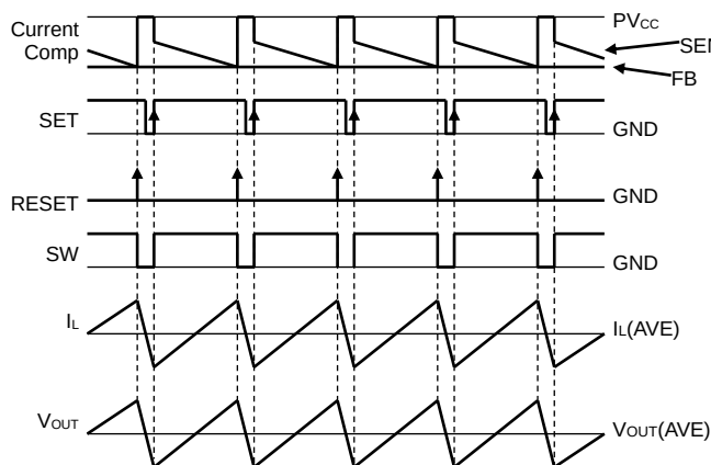
Figure 19. Diagram of Current Mode PWM Control
