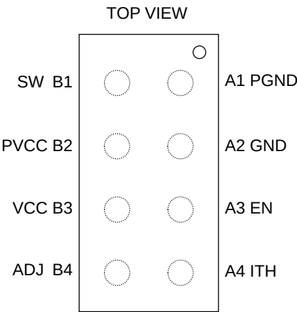
Figure 2. Pin Configuration
