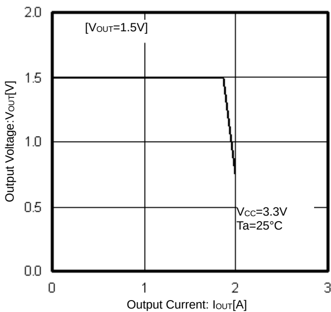
Figure 6. Output Voltage vs Output Current
