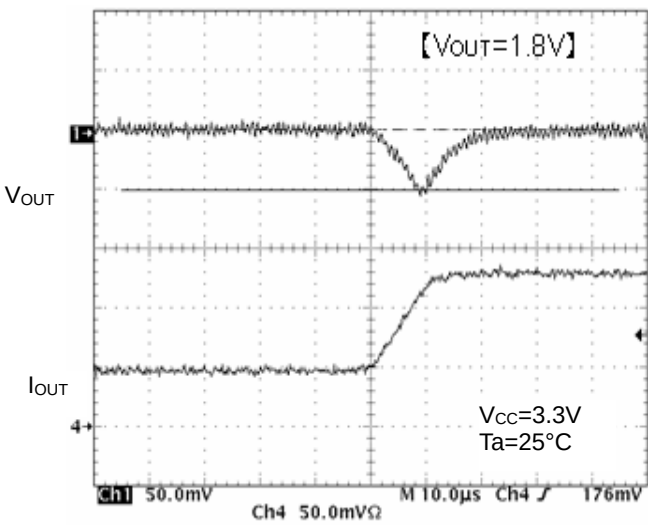
Figure 17. Transient Response (Io=50mA to 125mA , 10µs)
