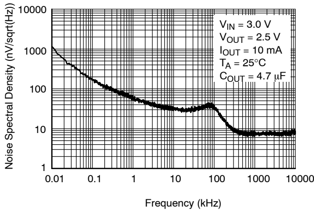
Figure 26. Output Voltage Noise Spectral Density for V_{OUT} = 2.5 V, C_{OUT} = 4.7 \mu F
