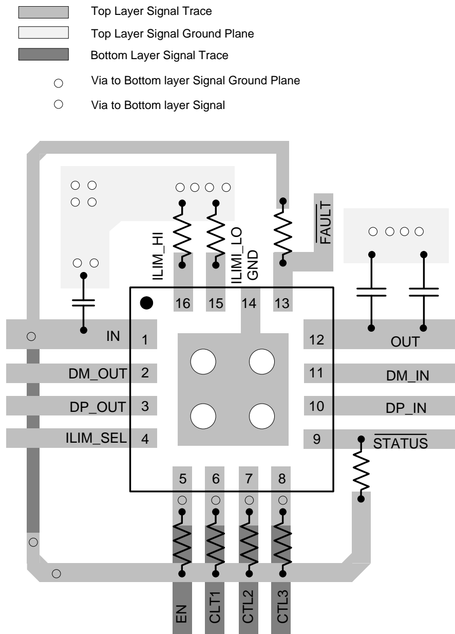
Figure 47. Layout Recommendation
