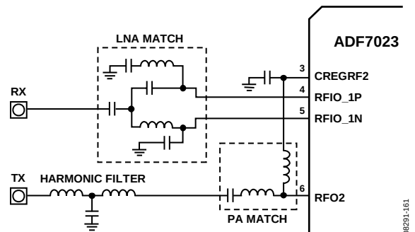
Figure 114. Separate Single-Ended PA and LNA Match
