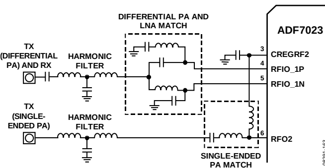
Figure 116. Matching Topology for Transmit Antenna Diversity
